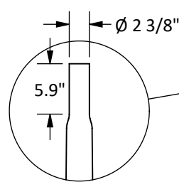
Standard Pole Top with 2 3/8" Tenon
