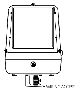
Wall Mounting
