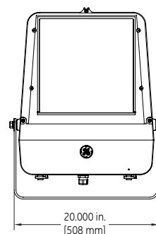
Trunnion Mounting
