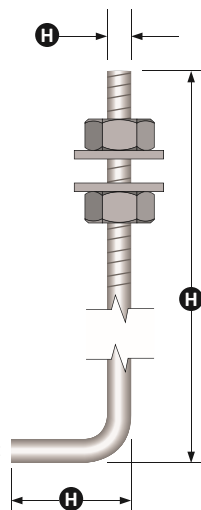
(4) Anchor Bolt
