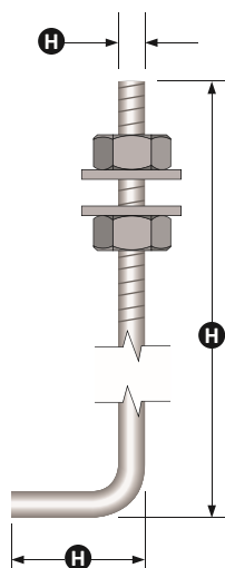
(4) Anchor Bolt
