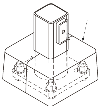
2 Piece Cover Finished to Match Pole
